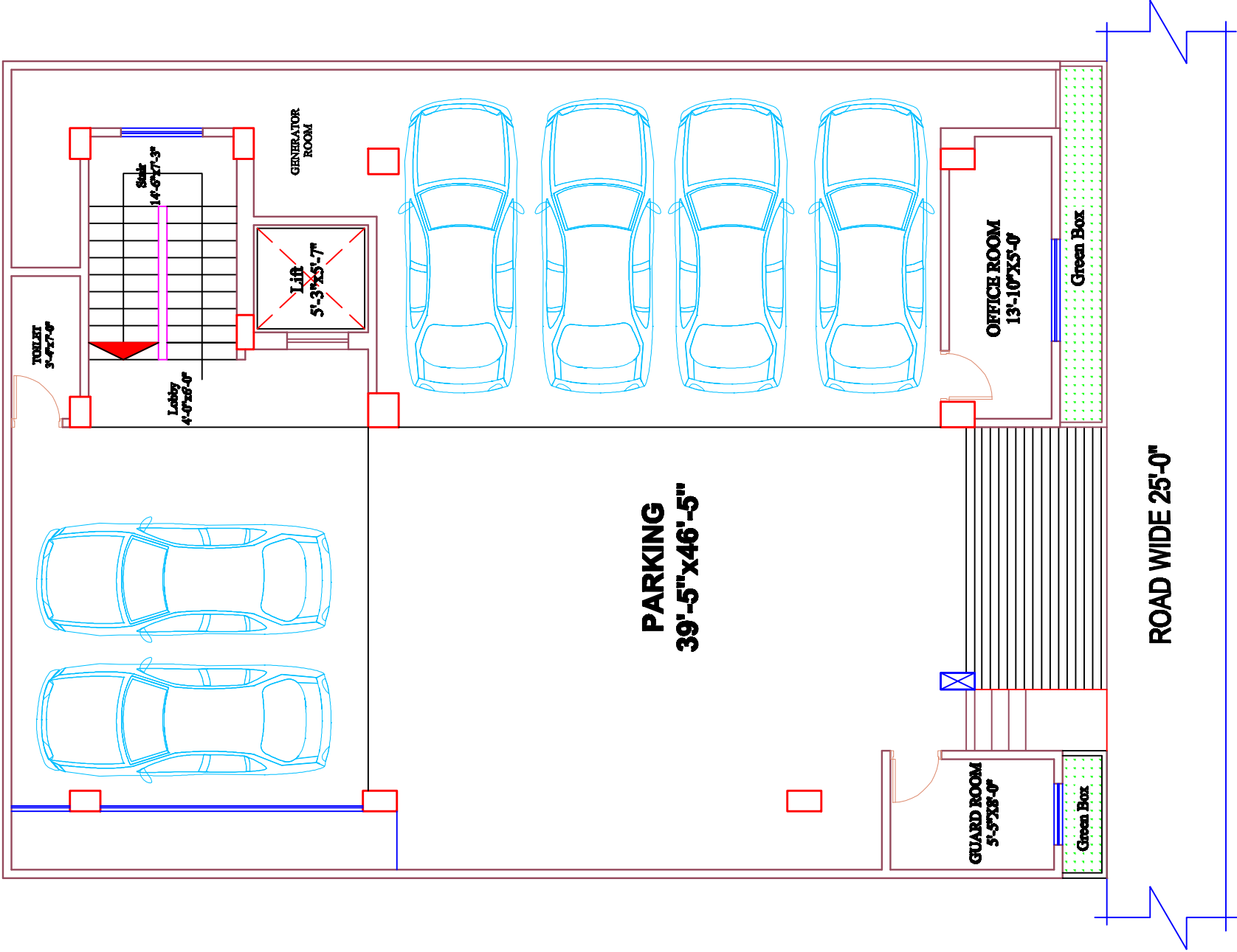
PARKING FLOOR PRESENTATION PLAN
